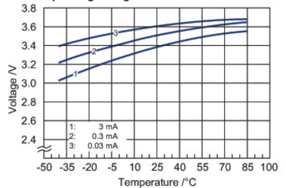
Operating Voltage
